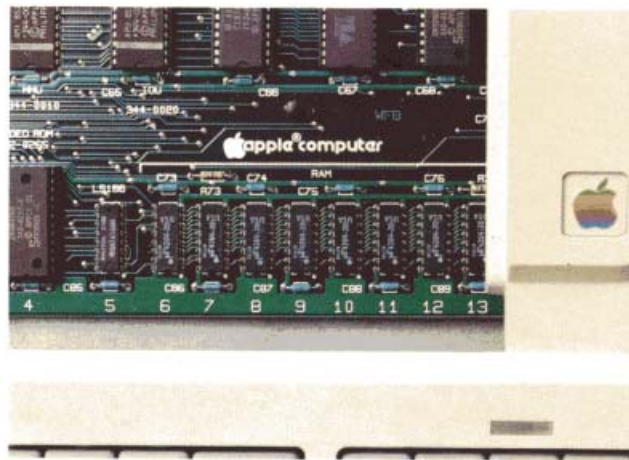
Figure 4-3 RAM chips
