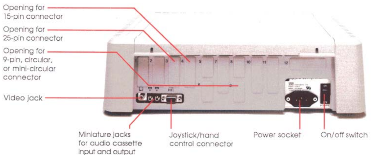
Figure 1-11 Back panel of the Apple IIe
