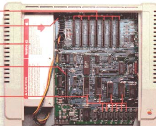
Figure 1-5 The Apple IIe main logic board
